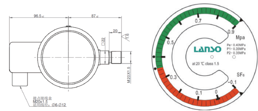
侧装度盘 (3点钟)
